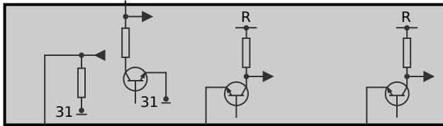
S29 Brake light switch
