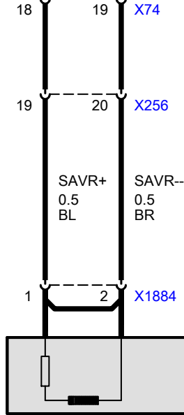
G15 Inflator assy for side airbag, passenger's door
