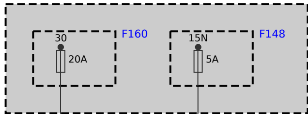
Z2 Fuse holder, rear
