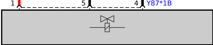
Y87 Valve block, driver's seat back- rest width adjustment
