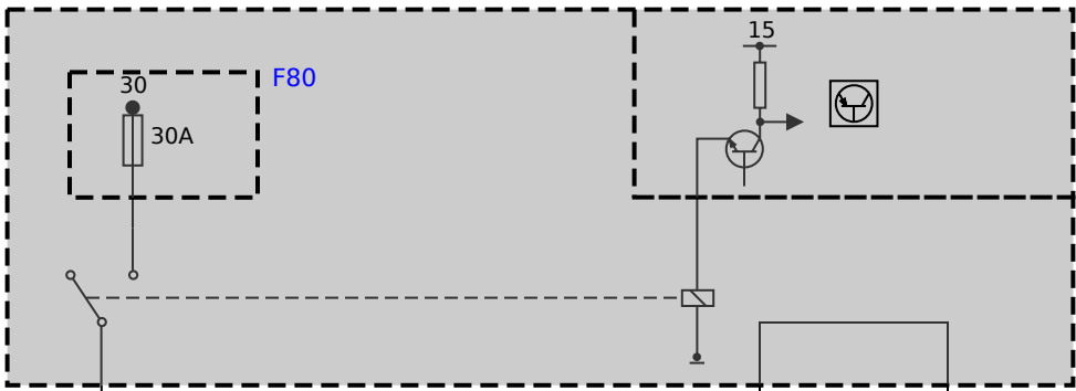
A174 Rear Electronic Module
